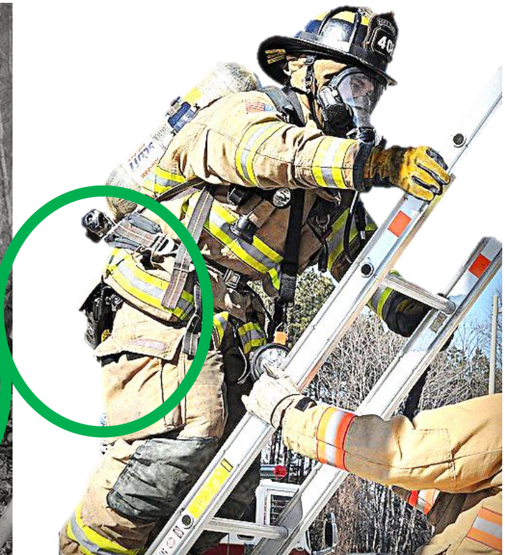
Figure 12 - Another example of the antenna canted away from the body naturally, eliminating up to 15-decibel loss over wearing it in the pocket.
